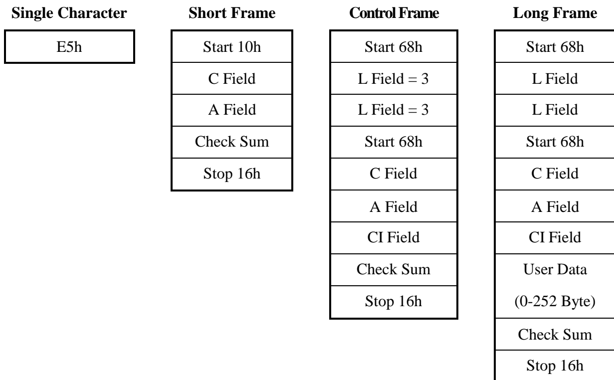
Fig. 13 Telegram Formats of the M-Bus Protocol
