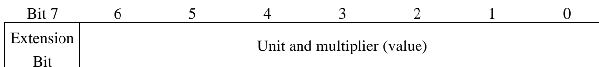
Fig. 23 Coding of the Value Information Field (VIF)
